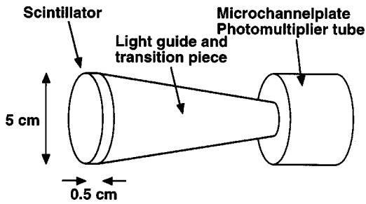
FIG. 2. Schematic of a typical current-mode neutron detector. The dimensions listed are for n ToF-6 and n ToF-17.
