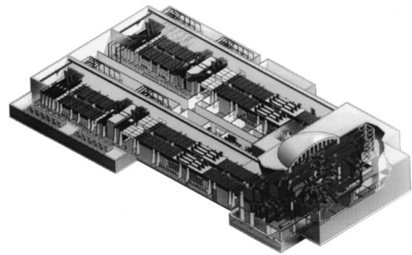
FIG. 1. The National Ignition Facility is a 192 beam, 2 MJ glass laser currently under construction at Lawrence Livermore National Laboratory.
