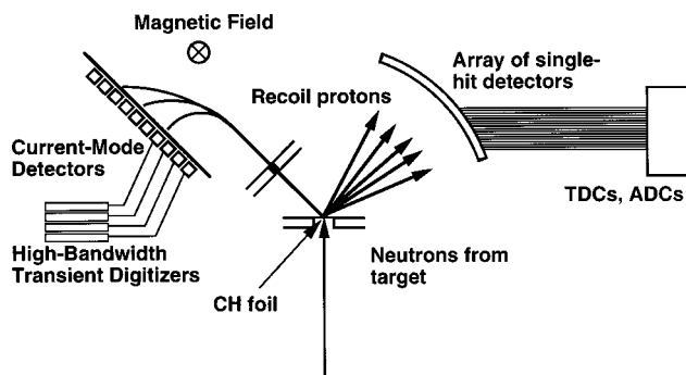
FIG. 8. Methods of measuring neutrons using recoil protons using apertured detectors to (left) select a single recoil angle and magnetic field to analyze the proton energy or (right) using detectors that measure the energy of each recoil proton.
