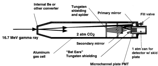
FIG. 5. Design for a gas Cerenkov detector that has been designed and fabricated for use on the Omega Laser Facility.
