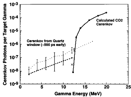
FIG. 4. Detection efficiency of the gas Cerenkov detector. The threshold can be adjusted by changing the gas pressure.
