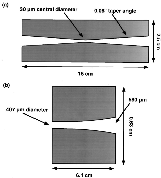
FIG. 7. Comparison of (a) a neutron pinhole that will be fielded on Omega high-yield implosion experiments and (b) a penumbral aperture used on Nova experiments.
