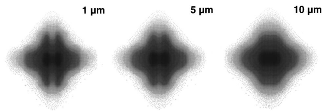
FIG. 6. Simulated neutron images from a NIF capsule that failed due to too large a flux asymmetry driving the capsule. At 10 \mu\text{m} resolution, the asymmetry of the implosion is seen, but details require higher spatial resolution.
