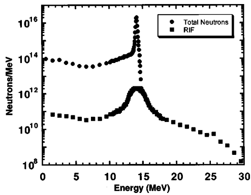
FIG. 3. Calculated tertiary [reaction-in-flight (RIF)] neutrons from a high-convergence NIF capsule as well as the total neutron spectrum.
