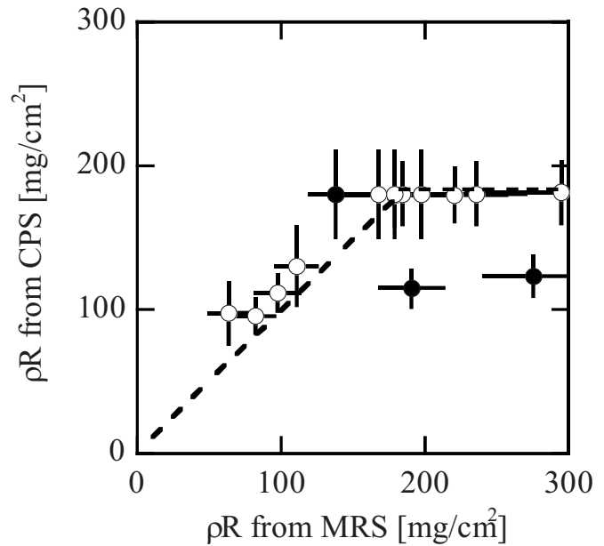
FIG. 7. \rho R inferred from CPS data as a function of \rho R inferred from MRS data. The open data points were obtained when the imploding capsule had a high-quality ice layer and was centered close to TCC, while the solid points were obtained when the imploding capsule had a poor ice layer and was significantly offset from TCC. As expected, the open data points are close to the symmetric-implosion line (dashed line). At \rho R values higher than \sim 180 mg/cm ^2 the assessment of the compression performance must rely on the MRS data, ice-layer data, and offset data, as the CPS technique has saturated. As shown by the solid data points, the poor ice layer and large offset have a detrimental impact on the \rho R symmetry of an implosion. This is also generally the case when the offset is larger than the hot-spot radius at peak compression.
