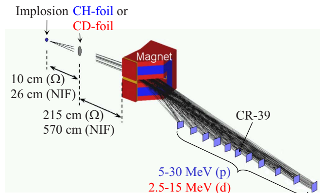
FIG. 1. (Color online) A schematic drawing of the MRS, including the CH (or CD) foil, magnet, and CR-39 detector array. The foil is positioned 10 and 26 cm from the implosion at OMEGA and the NIF, respectively; the magnet is positioned outside the target chamber on both facilities, i.e., 215 cm to the foil on OMEGA and 570 cm to the foil on the NIF. Important to the overall design is that the same magnet design is used in both the OMEGA-MRS and NIF-MRS. For detection of the forward scattered recoil protons (or deuterons) when using a CH foil (or CD foil), eleven and nine 7 \times 5 cm 2 CR-39 detectors are positioned at the focal plane in the OMEGA-MRS and NIF-MRS, respectively. The trajectories shown are for proton energies from 5 to 30 MeV, corresponding to deuteron energies from 2.5 to 15 MeV. The length of the detector plane is 166 and 84 cm for the OMEGA-MRS and NIF-MRS, respectively.
