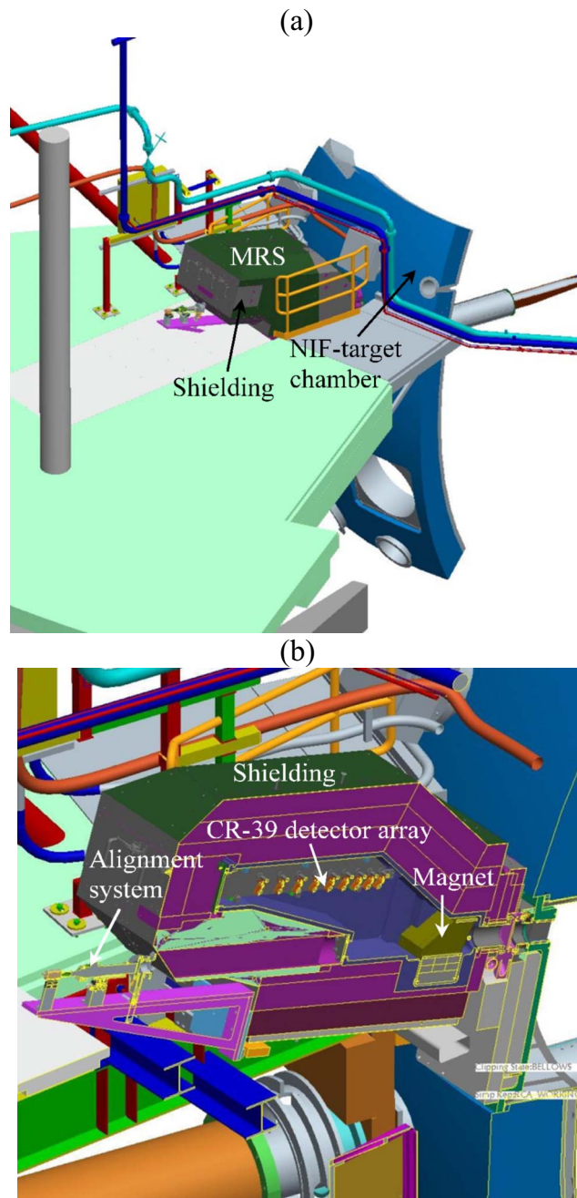
FIG. 2. (Color online) (a) An engineering drawing of the MRS positioned onto the NIF-target chamber at the 77^\circ – 324^\circ line-of-sight. For maximum suppression of the neutron-induced background, the CR-39 detector array is fully enclosed by \sim 6000 lb of polyethylene shielding and positioned in the shadow of the 60-cm-thick NIF-target chamber (50 cm of concrete and 10 cm of aluminum). (b) A vertical cross cut through the MRS illustrating the various components in the system, i.e., the magnet, CR-39 detector array, alignment system, and shielding. The diagnostic insertion manipulator (DIM) at 90^\circ – 315^\circ , not shown in these figures, will be used to the insert of the foil to a distance of 26 cm from the implosion.
