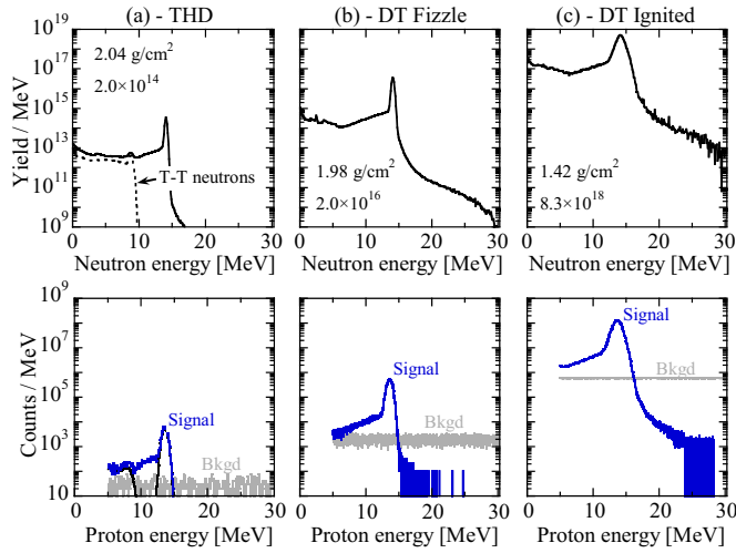
FIG. 8. (Color online) A set of LASNEX-simulated neutron spectra and associated MRS signal and background spectra for three different NIF implosions; (a) a low-yield THD implosion (the dashed line indicates the T–T neutron spectrum), (b) a fizzle DT implosion, and (c) an ignited DT implosion. The T–T neutron component in the two DT cases is insignificant and therefore not shown. The total \rho R and Y_n for each implosion are shown in each figure. These spectra were simulated for the MRS configured with a CH foil (Med-Res mode). The CCT, recently developed and now routinely used to analyze OMEGA-MRS data, was applied to determine the MRS signal and background spectra for the low-yield THD and fizzle DT implosions. For the ignited case, the SCT was applied to the data as the CCT is not effective at high track densities (Ref. 19). As shown by the spectra, excellent S/B is achieved for the dsf , T_i , and Y_n measurements.
