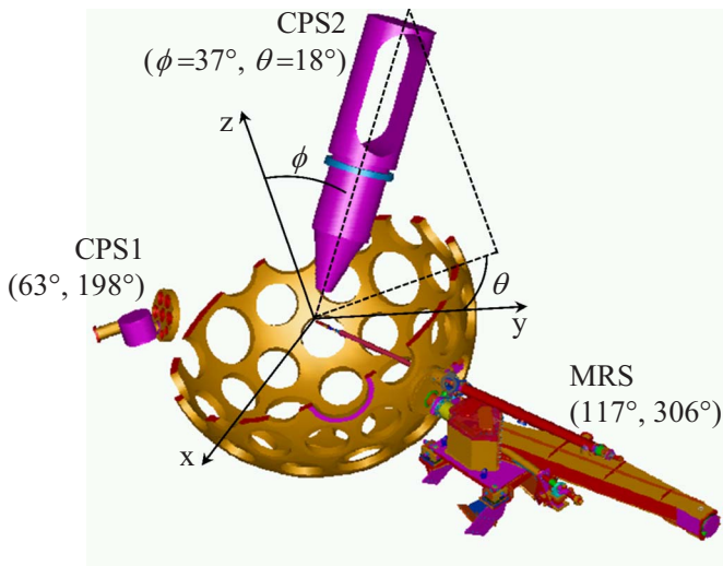
FIG. 3. (Color online) MRS, CPS1 and CPS2 on the OMEGA chamber. The MRS is shown here without the 2000-lb shielding that surrounds the diagnostic. The line of sight for each diagnostic is illustrated in terms of the polar angle \phi and azimuthal angle \theta . These spectrometers are used to measure the spectra of KO-Ds (CPS1 and CPS2) and downscattered neutrons (MRS) from which fuel \rho R and \rho R asymmetries in cryogenic DT implosions are inferred.
