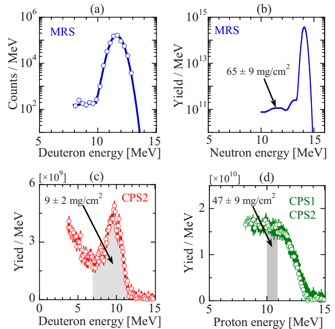
FIG. 4. (Color online) Integrated MRS and CPS data obtained for a series of eight CH-capsule implosions producing 1.6 \times 10^{14} primary neutrons (neutron-averaged T_i was 5.3 keV). In each shot, a capsule with a 15- \mu\text{m} -thick CH shell filled with 15 atm of DT gas was imploded with a 1 ns square pulse delivering \sim 23 kJ of laser energy. (a) The MRS-measured deuteron spectrum and fit to the measured spectrum, which are convolutions of the neutron spectrum and MRS-response function. In these measurements, the MRS was operated with a CD foil in Med-Res mode (see Table I). From the dsf value determined from the modeled neutron spectrum, shown in (b), a total \rho R (fuel+shell) of 65 \pm 9 mg/cm 2 was inferred. Data points at neutron energies below 10 MeV were excluded in the analysis as they are comprised primarily of T–T neutrons. (c) CPS2-measured spectrum of KO-Ds produced in the fuel. From the yield in the high-energy peak (Ref. 20) (marked gray) a fuel \rho R of 9 \pm 2 mg/cm 2 was inferred. (d) CPS1 and CPS2-measured spectra of knock-on protons (KO-P) produced in the shell. From the yield in the plateau (Ref. 20) (marked gray) a shell \rho R of 47 \pm 9 mg/cm 2 was inferred. A total \rho R of 56 \pm 10 mg/cm 2 was thus determined from the CPS1 and CPS2 data. Given that \pm 15\% \rho R asymmetries are typically observed for this type of implosion, the \rho R values determined from the MRS and CPS data are in good agreement.
