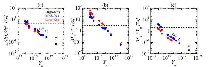
FIG. 9. (Color online) Statistical measurement uncertainty for dsf (a), T_i (b), and Y_n (c) as a function of neutron yield when the MRS is operating in High-Res, Med-Res, and Low-Res modes. Thirteen implosions were used in these calculations. The relative requirements illustrated in Table II are indicated by the dashed lines.
