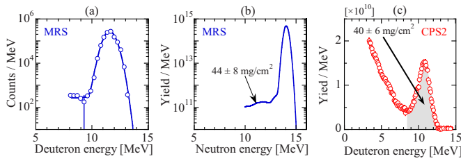
FIG. 5. (Color online) Integrated MRS and CPS data obtained for a series of five CD-capsule implosions producing 2.6 \times 10^{14} primary neutrons (neutron-averaged T_i was 8.0 keV). In each shot, a capsule with a 10- \mu\text{m} -thick CD shell filled with 10 atm of DT gas was imploded with a 1 ns square pulse delivering \sim 23 kJ of laser energy. (a) The MRS-measured deuteron spectrum and fit to the measured spectrum, which are convolutions of the neutron spectrum and MRS-response function. In these measurements, the MRS was operated with a CD foil in Med-Res mode (see Table I). From the dsf value determined from the modeled neutron spectrum, shown in (b), a total \rho R (fuel+shell) of 44 \pm 8 mg/cm ^2 was inferred. Data points at neutron energies below 10 MeV were excluded in the analysis as they are primarily comprised by T-T neutrons. (c) CPS2-measured illustrating a spectrum of KO-Ds produced in the fuel and shell. From the yield in the high-energy peak (Ref. 20) (marked gray) a total \rho R of 40 \pm 6 mg/cm ^2 was inferred, which is in excellent agreement with the \rho R value determined from the MRS.
