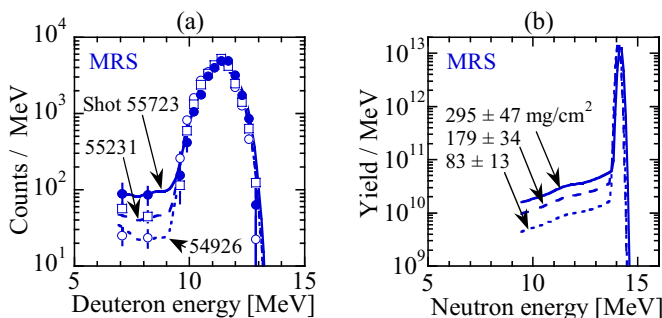
FIG. 6. (Color online) MRS data obtained for three low-adiabat cryogenic DT implosions producing neutron yields in the range of 2 \times 10^{12} – 4 \times 10^{12} (neutron-averaged T_i was \sim 2 keV for these implosions). (a) MRS-measured deuteron spectra for the three implosions and fits to the measured spectra, which are convolutions of the underlying neutron spectra and the MRS-response function. In these measurements, the MRS was operated with a CD foil in Low-Res mode (see Table I). From the modeled neutron spectra, shown in (b), dsf values and thus \rho R s were determined for the three implosions. A \rho R of 83 \pm 13 mg/cm ^2 was determined for shot 54926 (imploded with an alpha-3 laser pulse), which is \sim 40\% of the 1D value—a result of a poorly designed laser drive. A \rho R of 179 \pm 34 mg/cm ^2 was determined for shot 55231 (imploded with an alpha-3 laser pulse). In this case, the picket pulses in front of the main laser drive were tuned correctly, resulting in a \rho R value closer to the 1D value of 220 mg/cm ^2 . For shot 55723, a \rho R of 295 \pm 47 mg/cm ^2 was determined (imploded with an alpha-2 laser pulse), which is in agreement with the 1D \rho R value considering the error bar. An optimal multiple-picket laser drive was applied in this case as well.
