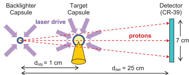
Fig. 1. Schematic of the experimental setup. A short (130-ps), monoenergetic (energy linewidth \Delta E/E < 3\% ), quasi-isotropic pulse of 15.0-MeV \text{D}^3\text{He} fusion protons is generated by laser implosion of a backlighter capsule filled with \text{D}_2 and ^3\text{He} gas. The \sim 3 \times 10^8 protons emitted from the 45- \mu\text{m} full width at half maximum source region interact with matter and electromagnetic fields in a cone-in-shell capsule implosion. The position and energy of every proton reaching the detector are individually recorded on CR-39, encoding the details of the matter and field distributions surrounding the target capsule.
