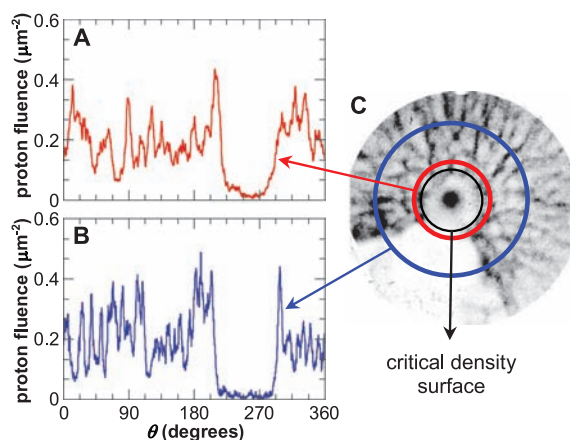
Fig. 5. Circular lineouts of proton fluence obtained from OMEGA shot 46529 at radii of 430 \text{ }\mu\text{m} (A) and 860 \text{ }\mu\text{m} (B). The filamentary structures represent a 2D projection of a 3D field structure that originates inside the critical density surface (C).
