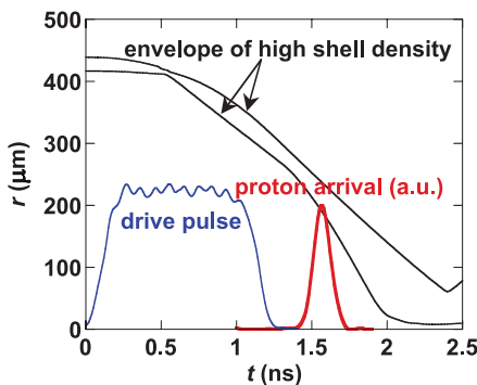
Fig. 2. Cone-in-shell capsule drive pulse (blue line), simulated (17) shell trajectory (black lines), and experimental backlighter proton arrival time t (red line). Simulations predict that the shell has compressed from its original radius by about a factor of two, and the \rho R has doubled to 5 \text{ mg/cm}^2 when the backlighter protons arrive at 1.56 ns (OMEGA shot 46529). a.u., arbitrary units.
