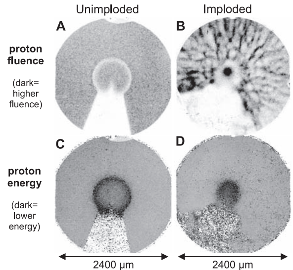
Fig. 3. Images of a 430- \mu\text{m} -radius spherical plastic capsule with attached Au cone, before and during implosion. (A and C) The unimploded capsule used in OMEGA shot 46531. (B and D) A capsule at 1.56 ns after the onset of the laser drive (OMEGA shot 46529). The dark areas correspond to regions of higher proton fluence [in (A) and (B)] and regions of lower proton energy [in (C) and (D)]. The energy image values in the region shadowed by the cone are mostly noise because very few protons were detected in that region. See lineouts in Figs. 4 and 5 for image values.
