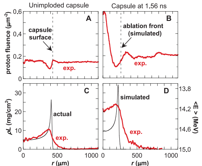
Fig. 4. Experimental (exp.) radial lineouts (red lines) of proton fluence and \rho L from Fig. 3. All lineouts are averaged over the azimuth, excluding the region of the cone shadow. (A and C) Unimploded capsule of OMEGA shot 46531. (B and D) Capsule of OMEGA shot 46529, 1.56 ns after start of laser drive. The fluence lineout (A) shows the effects of angular scattering through the limb of the capsule shell. In (B), angular scattering effects alone are insufficient to explain the peak at r = 0 . A radial electric field of \sim 10^9 \text{ V/m} is necessary to focus the protons to the extent observed. In (C) and (D), radial lineouts of the mean energy images in Fig. 3 were converted to \rho L . Also displayed are the actual \rho L (C) and simulated \rho L (D), assuming no angular scattering (black line). \rho R is given by \rho L/2 at r = 0 .
