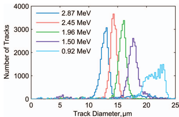
FIG. 1. Distribution of proton track diameters on CR-39 for different incident proton energies, replacing Figure 1(c) in the original paper. 1
