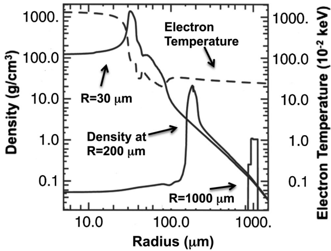
FIG. 1. Shell density profiles (solid curves) are shown as a function of shell radius at initial position (right-hand side curve), during implosion at radius of 200 \mu\text{m} (middle curve), and at the onset of ignition at a radius of 30 \mu\text{m} (left-hand side) with an electron temperature profile at the onset of ignition shown by a dashed curve.
