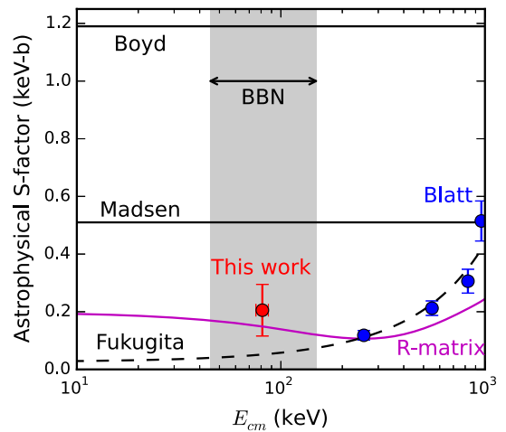
FIG. 4. Astrophysical S factor for the reaction \text{T}(\text{}^3\text{He}, \gamma)\text{}^6\text{Li} measured in this work, compared to previous data [9] and constant values used in BBN theory [3,7]. The total uncertainty for this measurement (statistical and systematic) is shown. The energy range of interest to BBN, 45–150 keV, is shown by the shaded region.
